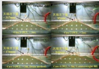
浸透流を考慮したため池堤体の遠心力場での模型振動実験 Centrifuge model test on seepage-seismic coupled behavior of a reservoir embankment
